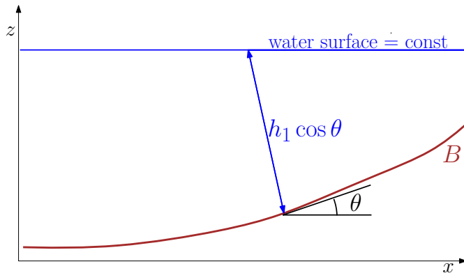
Figure 1.2: Diagram depicting the “lake-at-rest” steady-state. In the absence of a lower layer, the system reduces to a single-layer shallow water system.
