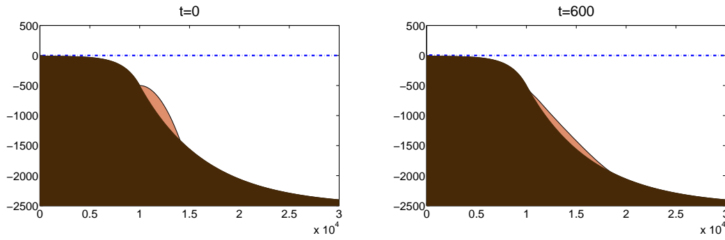
Figure 4.6: Initial condition and solution at t = 600 . The lower layer slides down the hill and stops due to the friction between the lower layer and non-errodible bottom B . Surface waves cannot be seen at this zoom level.
