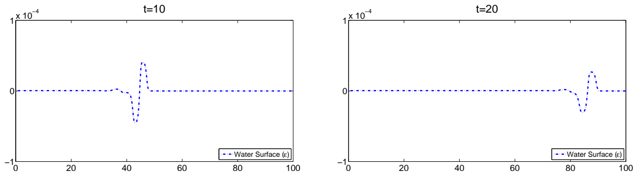
Figure 4.10: The same simulation as in Figure 4.9, but shown on a larger domain and at later times.
