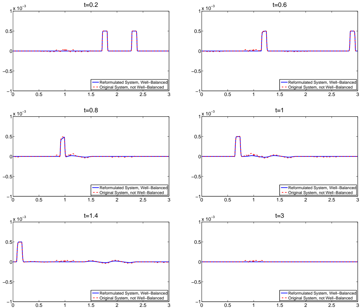
Figure 4.2: Solutions (the water surface) of (1.1) using the non-well-balanced scheme and of (2.2) using our well-balanced scheme with the same bottom topography and initial data given by (4.1) and (4.2) with \eta_1 = 10^{-3} and \eta_2 \equiv 0 ; \Delta x = 1/800 . The well-balanced scheme is oscillation-free and results in a physically relevant steady state whereas the non-well-balanced scheme develops nonphysical oscillations.
