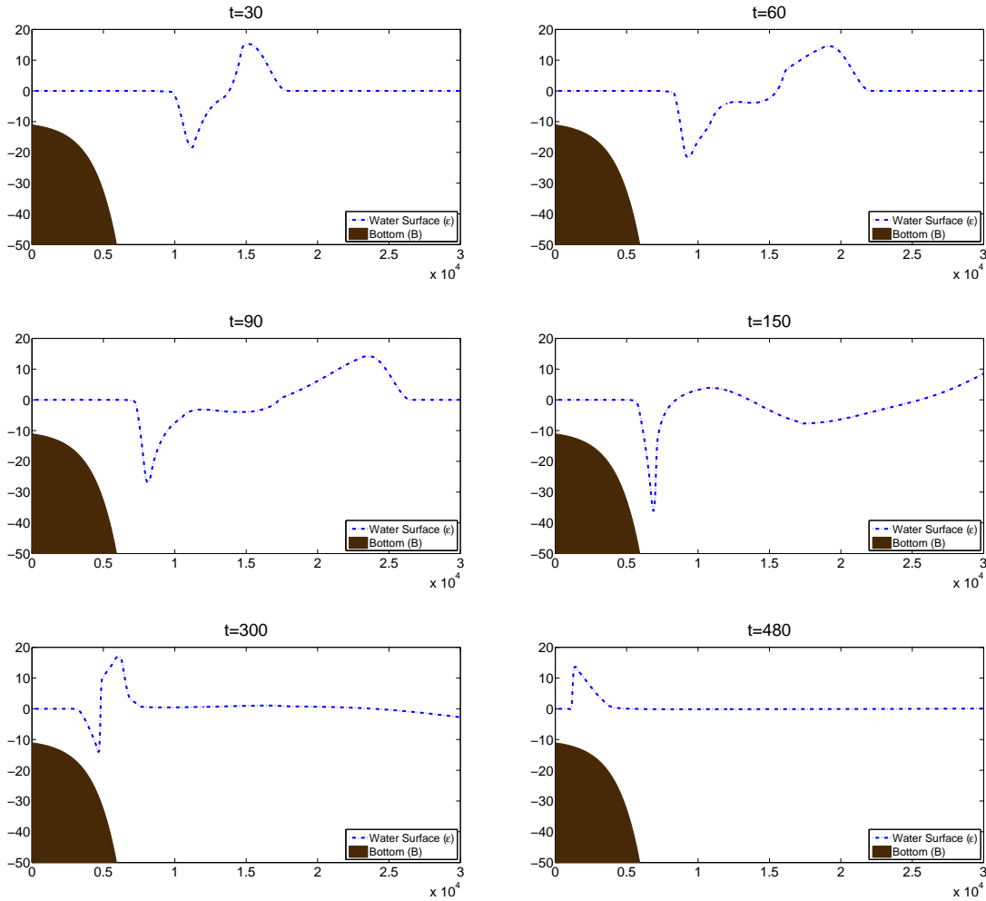
Figure 4.7: Zoomed time snapshots of the solution of (2.2) with the initial condition and bottom function given by (4.6) and (4.5), respectively.
