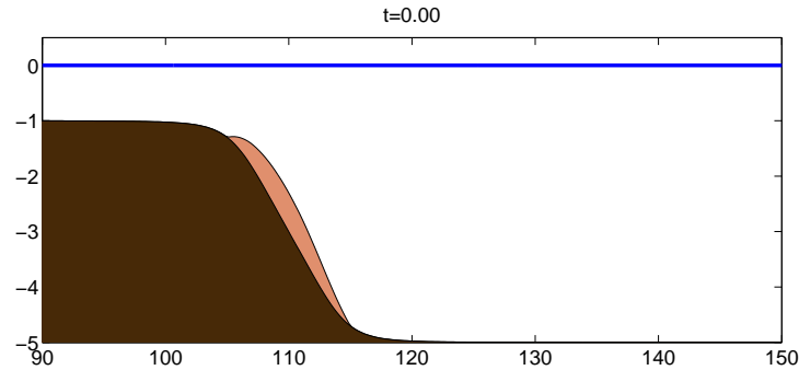
Figure 4.11: Bottom topography and initial condition given by (4.9) and (4.10), respectively. There is a small ridge formed by the sediment layer that deforms and generates small surface waves.
