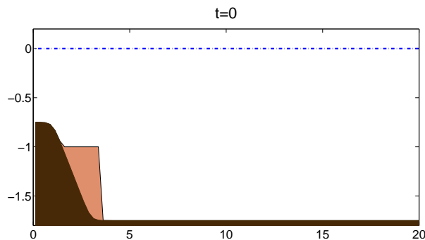
Figure 4.8: Bottom topography and initial condition given by (4.7) and (4.8), respectively. There is a small ridge formed by the sediment layer that deforms and generates small surface waves.
