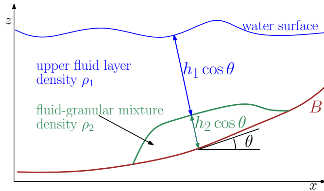
Figure 1.1: Diagram depicting the physical setting for the model. The fluid-granular layer with density \rho_2 and depth h_2 sits atop a non-erodible bottom B . A fluid layer with density \rho_1 sits atop the lower layer and the bottom.
