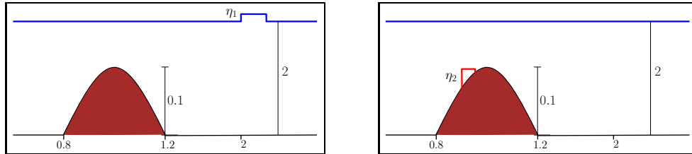
Figure 4.1: Initial data for small perturbation test problems as described by (4.1) and (4.2). For the solutions shown in Figures 4.2 and 4.3, \eta_1 = 10^{-3} and 0.014 \leq \eta_2 \leq 0.05 , so these pictures are not to scale.
