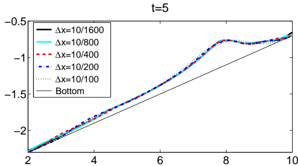
Figure 4.5: Zoom of the interface between the upper and lower layers at t = 5.0 .
