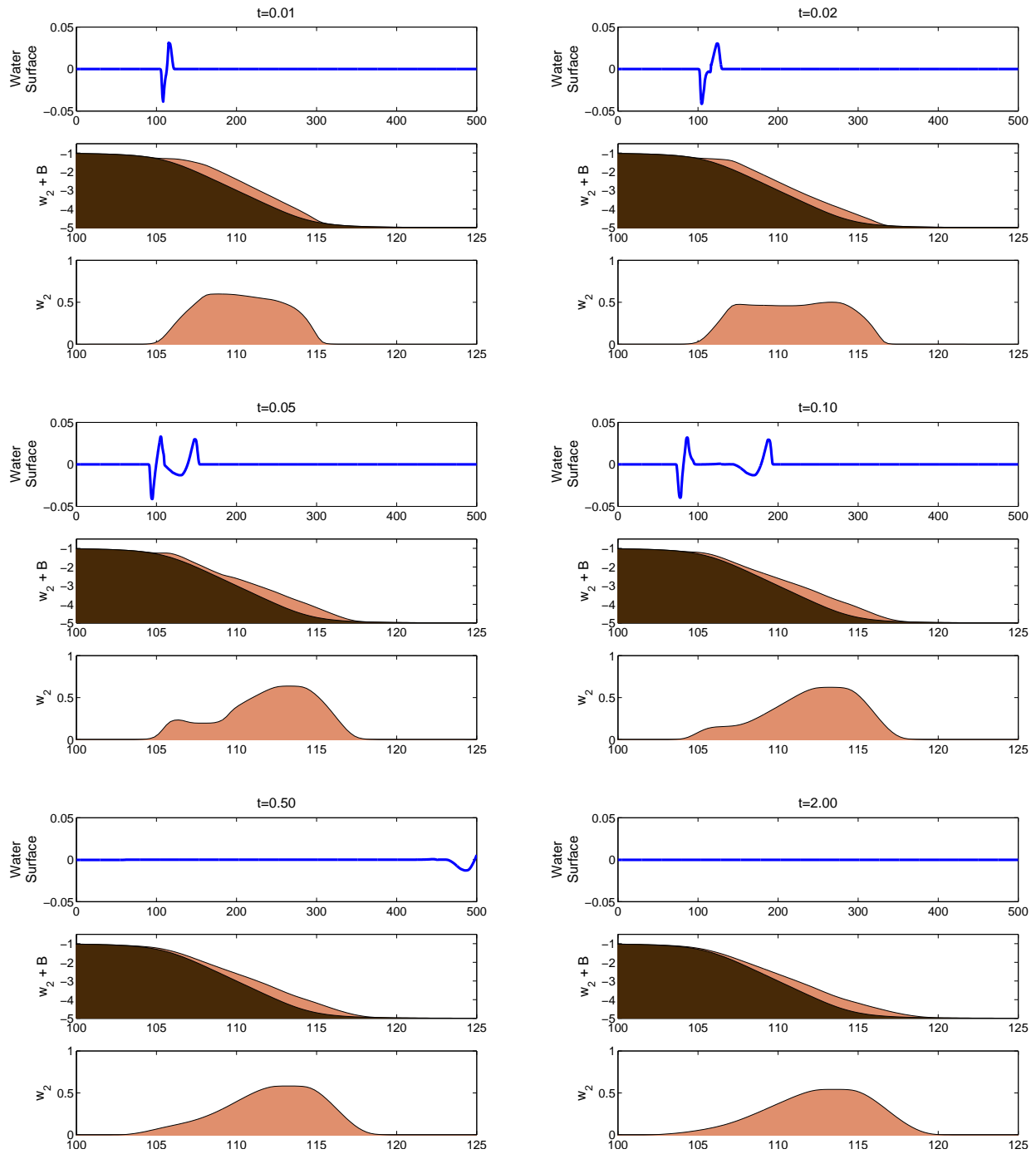
Figure 4.12: Solution (the water surface, the lower layer atop the bottom, and just the lower layer) of tsunami-like wave generation simulation at different time levels. The submarine landslide creates small surface waves that are undetectable when zoomed out. Our new scheme is able to capture the small wave with characteristic tsunami shape. The solution is computed on a computational domain 0 < x < 500 using \Delta x = 0.25 (the plots of the lower layer are zoomed to 100 \leq x \leq 125 ).
