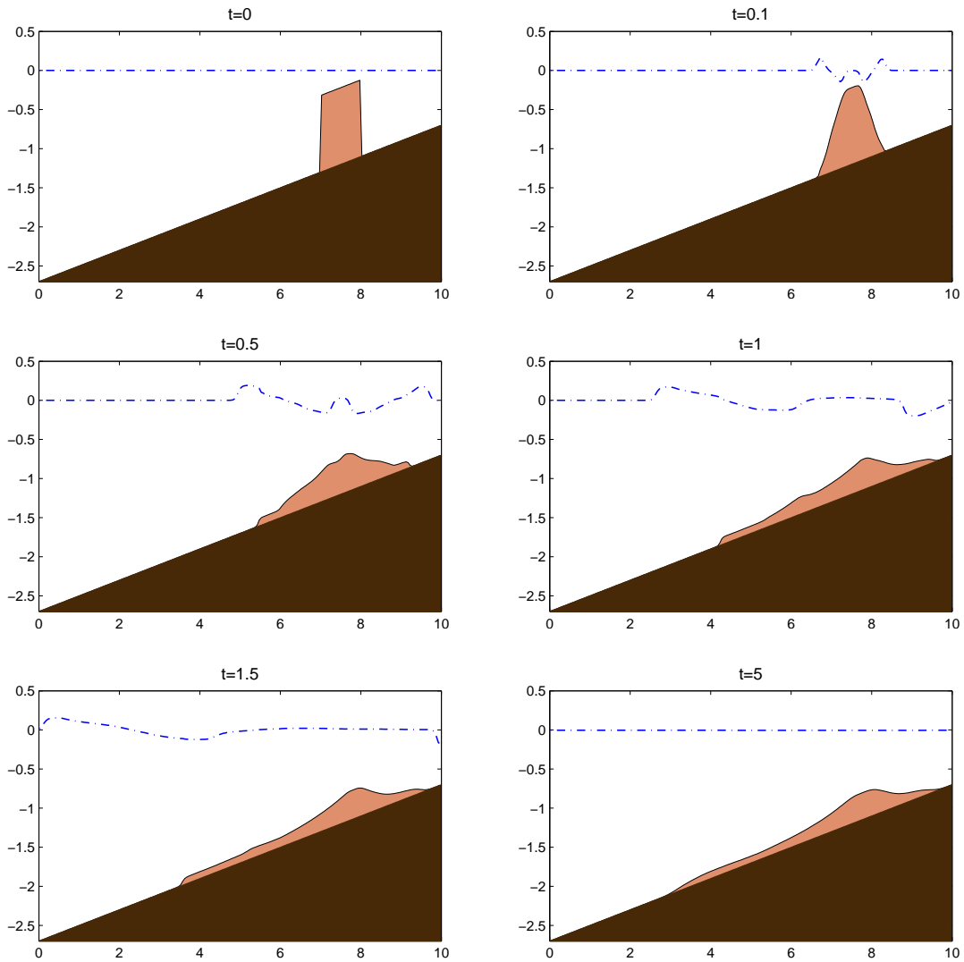
Figure 4.4: Time snapshots of the solution (the water surface, sediment layer, and bottom) of (2.2), (4.3), (4.4) with \Delta x = 0.05 . The deformation due to gravity in the lower layer creates large waves on the water surface. The lower layer slides downhill and stops due to friction between the material and the non-erodible bottom B .
