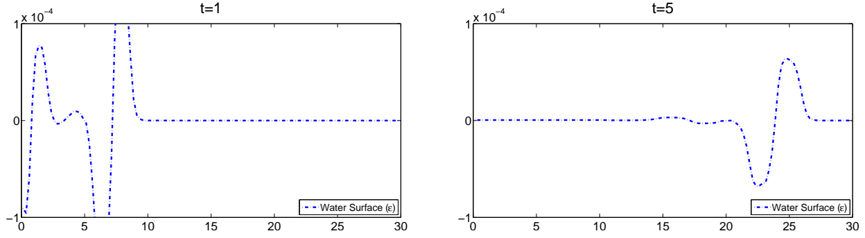
Figure 4.9: Solution (the water surface) of tsunami-like wave generation simulation at different time levels. The relatively small submarine landslide creates very small surface waves that are undetectable when zoomed out. Our new scheme is able to capture the very small wave with characteristic tsunami shape. The solution is computed on a computational domain 0 < x < 100 using \Delta x = 0.25 (the plots are zoomed to 0 \leq x \leq 30 ).
