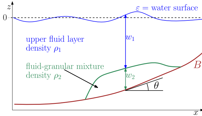
Figure 2.1: Diagram depicting the variables in the new system. The z -coordinate is shifted so that the bottom B is negative and the water surface reference level is 0. In practical applications, this ensures that the water surface \varepsilon is small since it is close to the reference level (dashed line).
