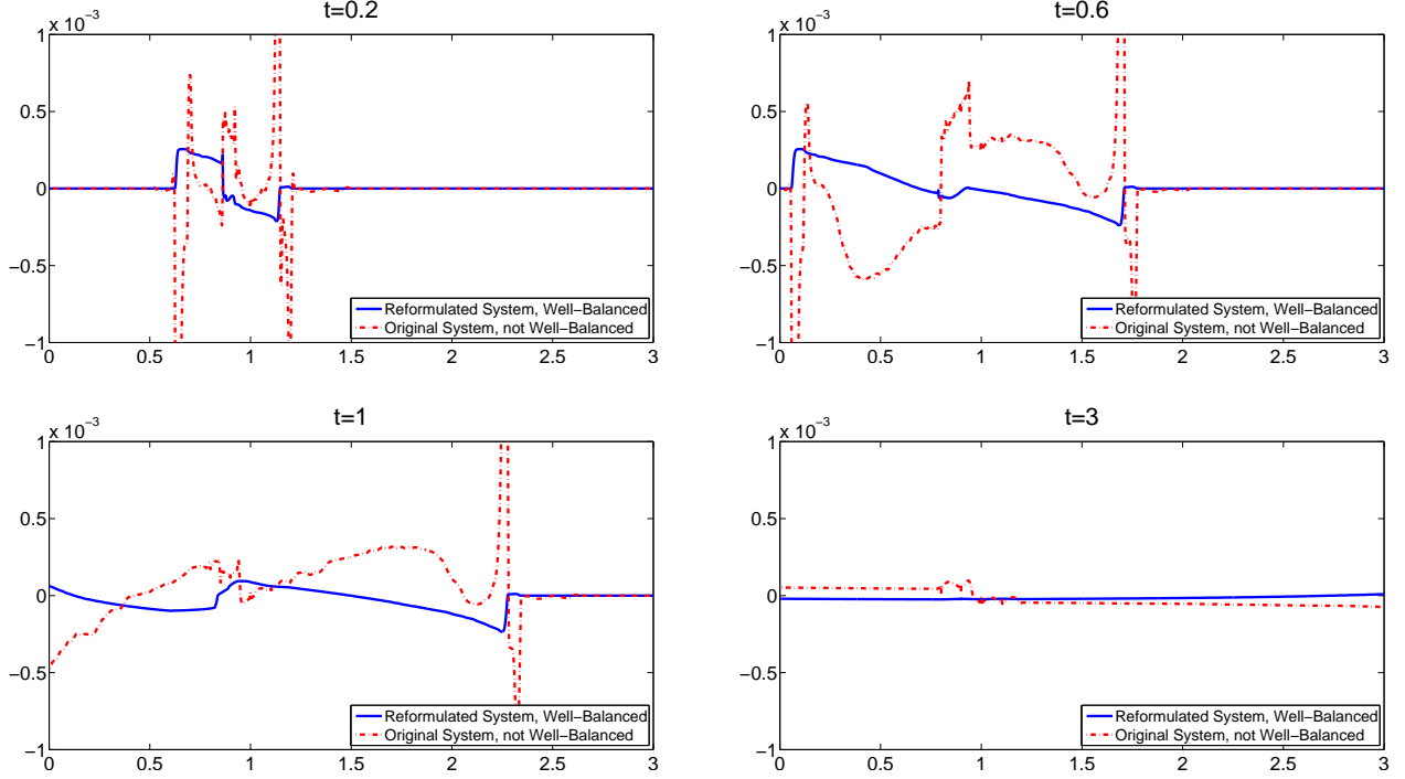
Figure 4.3: Solution (the water surface) of (1.1) using a non-well-balanced scheme and of (2.2) using our well-balanced scheme with the same bottom topography and initial data given by (4.1) and (4.2) with \eta_1 \equiv 0 and \eta_2 - 1.9 - B(x) ; \Delta x = 1/800 . Even though the well-balanced scheme develops small oscillations, it results in a physically relevant steady state whereas the non-well-balanced scheme produces physically irrelevant solution.
